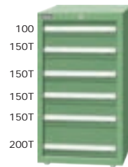
EA-10062T H1000xW566xD607 EB-10062T H1000xW718xD607 ED-10062T H1000xW718xD759
