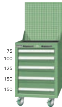
EA-7052MA H1380xW566xD640 EB-7052MA H1380xW718xD640
